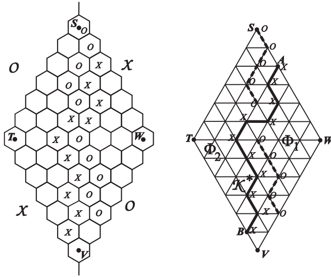
Figure 7: Hex board of size 7 and its dual graph
