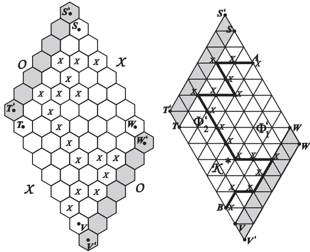
Figure 8: The widened hex board and its dual graph
