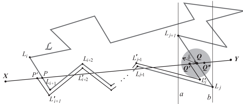
Figure 5: The values n(Q', \mathcal{L}) and n(Q'', \mathcal{L}) are of opposite parity
