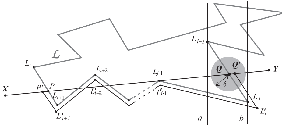
Figure 4: The broken line P'L'_{i+1} \dots L'_jQ' is “close” to the broken line PL_{i+1} \dots L_jQ
