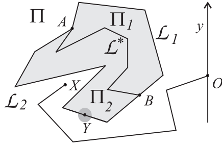
Figure 6: Polygon case of the Theta-Curve Theorem
