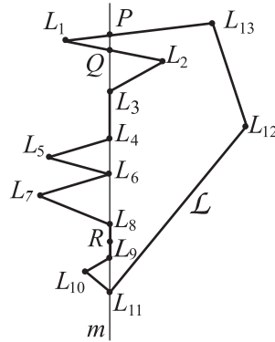
Figure 2: The proper points and proper sides of the intersection of \mathcal{L} and m are P, Q, L_{11} and [L_3L_4]
