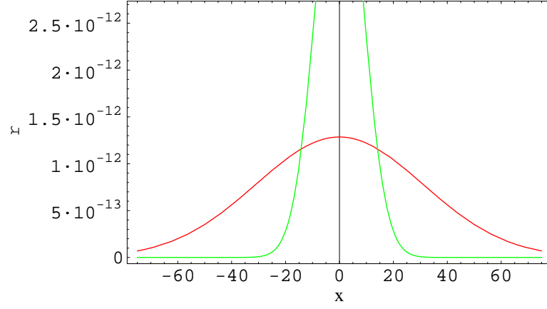
Figure 2: The probability density \rho \equiv r is plotted as a function of x'' \equiv x for \pi^0 and K^0 (upper curve at x = 0 )
