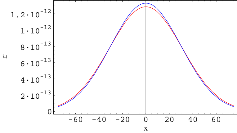
Figure 1: The probability density \rho \equiv r is plotted as a function of x'' \equiv x for \pi^\pm (upper curve at x = 0 ) and \pi^0
